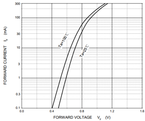
Forward current ( I_F ) vs Forward voltage ( V_F )
