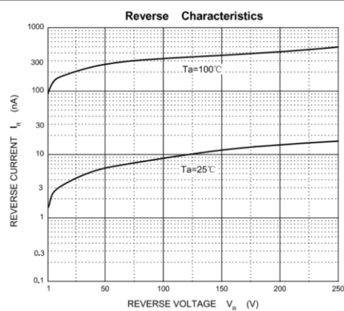
Reverse current ( I_R ) vs Reverse voltage ( V_R )
