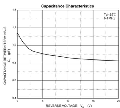
Capacitance Characteristics
