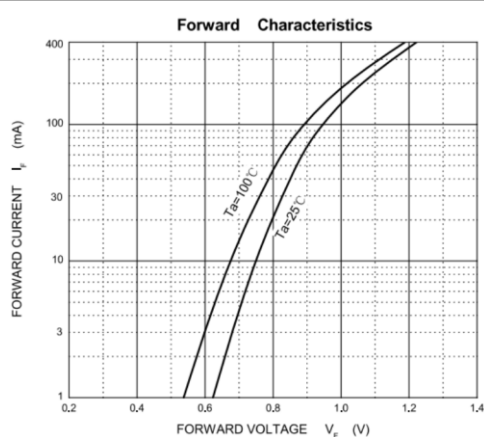
Forward current ( I_F ) vs Forward voltage ( V_F )
