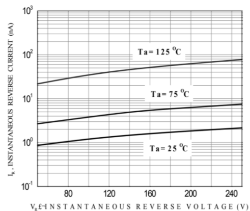
Reverse current ( I_R ) vs Reverse voltage ( V_R )
