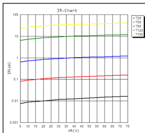
Reverse current ( I_R ) vs Reverse voltage ( V_R )
