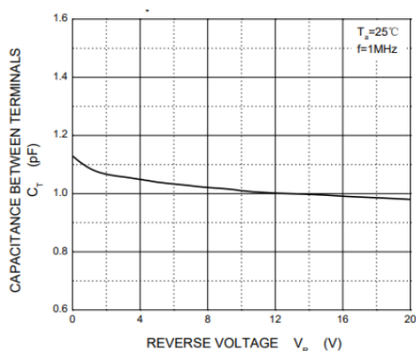
Capacitance Characteristics
