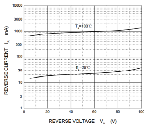
Reverse current (I R ) vs Reverse voltage (V R )
