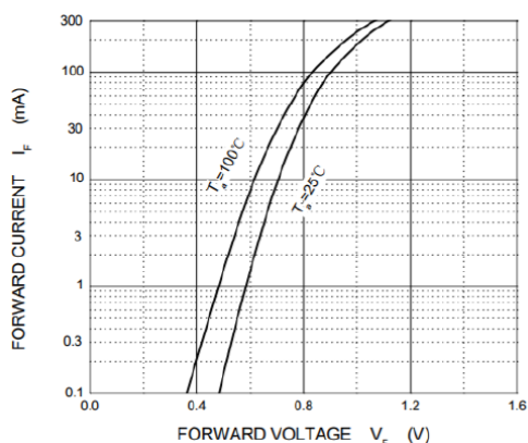
Forward current (I F ) vs Forward voltage (V F )
